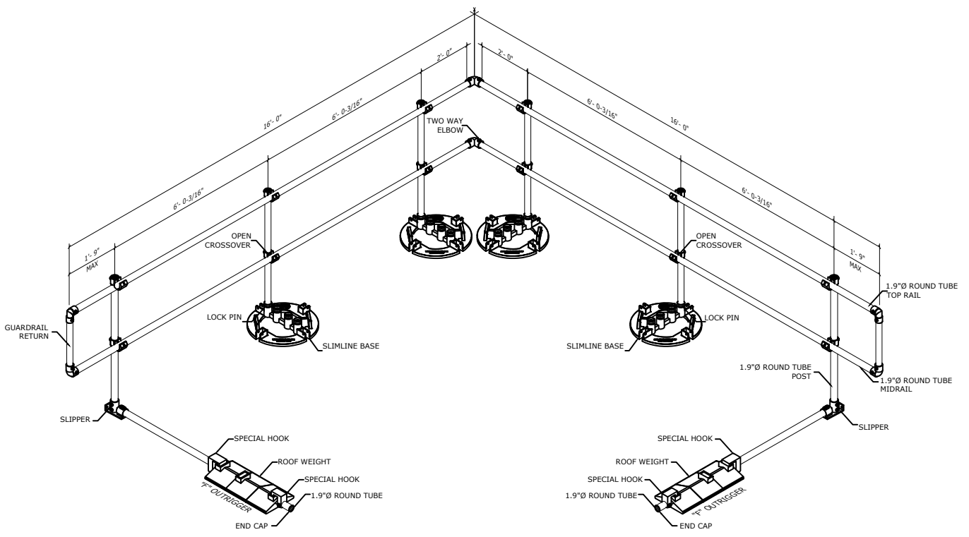
ISOMETRIC
