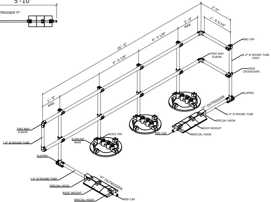
ISOMETRIC
