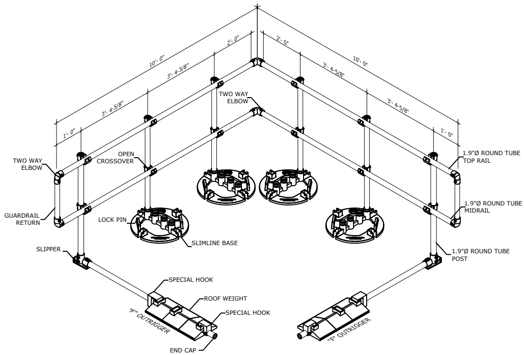
ISOMETRIC
