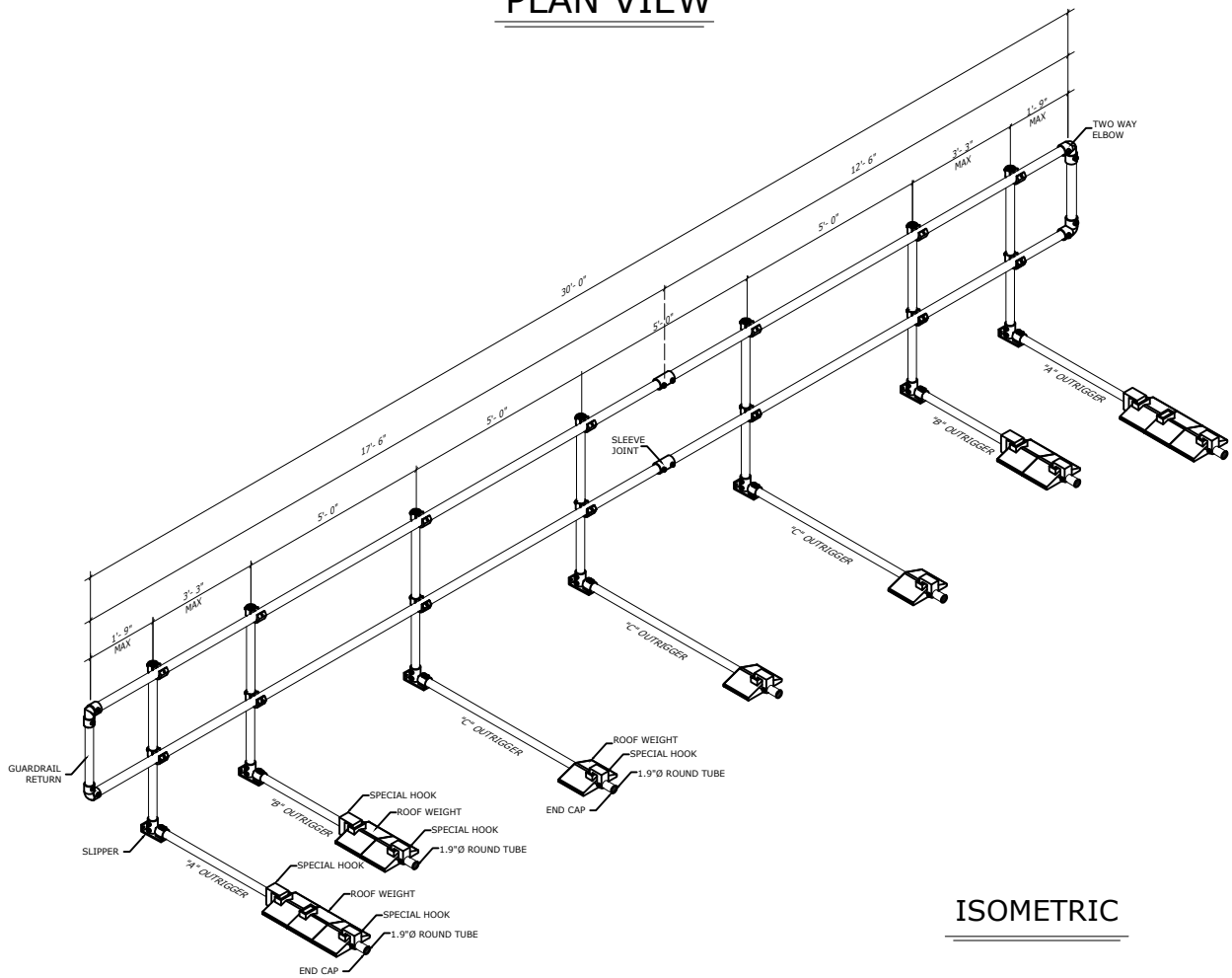
PLAN VIEW
