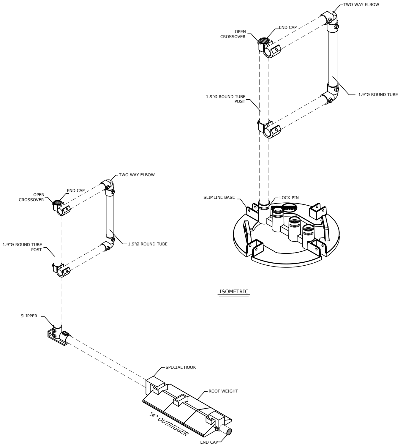
ISOMETRIC
